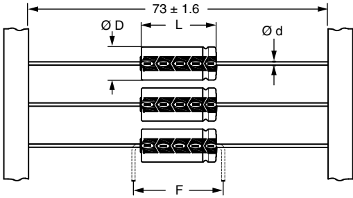
Form BR: Taped on reel Case \varnothing D \times L = 6.5 \text{ mm} \times 18 \text{ mm} to 15 \text{ mm} \times 30 \text{ mm} Form BA: Taped in box (ammopack) Case \varnothing D \times L = 6.5 \text{ mm} \times 18 \text{ mm} to 10 \text{ mm} \times 25 \text{ mm}
