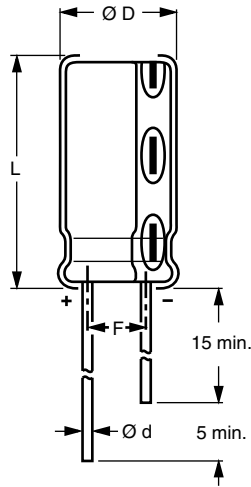
Fig. 2 - Form CA: Longs leads
