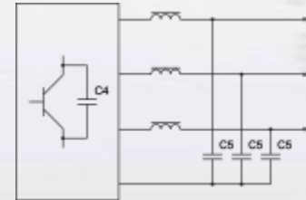
AC-Filter
