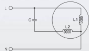
Typical Circuit
