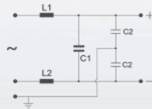
Typical Circuit
