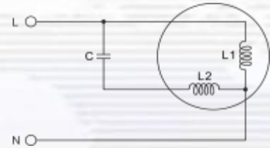
Typical Circuit
