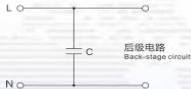
Typical Circuit
