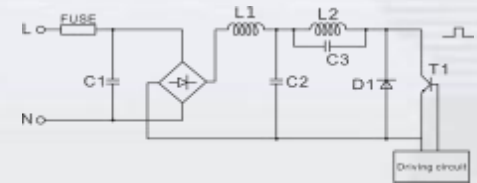
Typical Circuit
