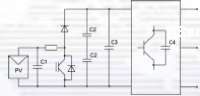
Snubber
